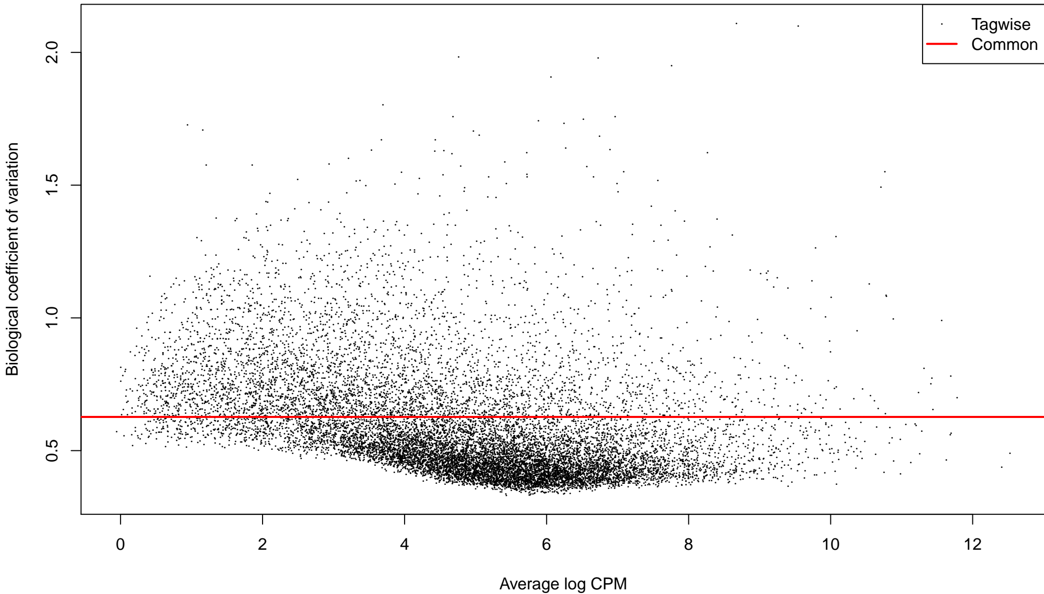
Plot of Estimated Dispersions
