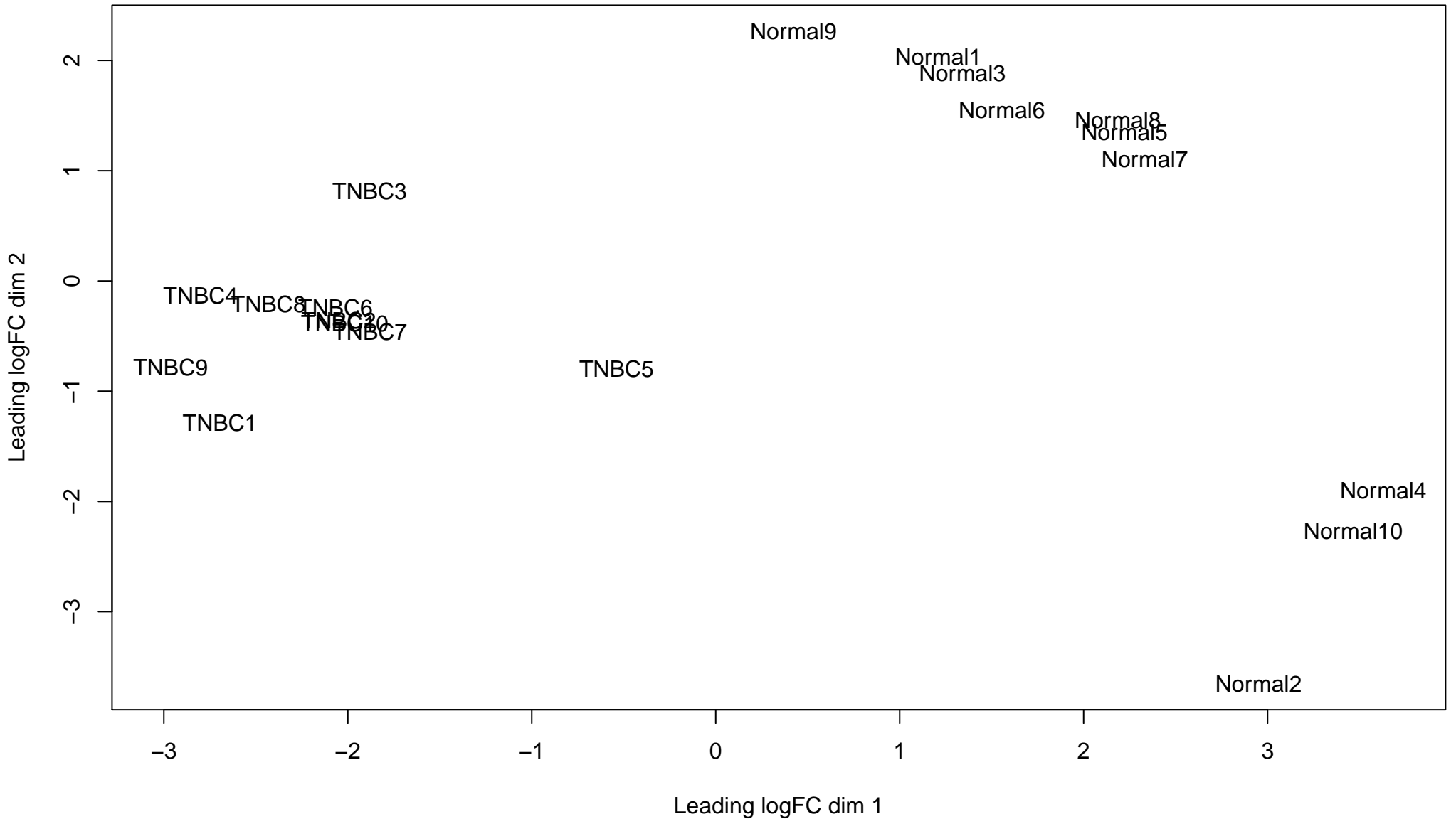
MDS Plot for TMM Normalized Count Data
